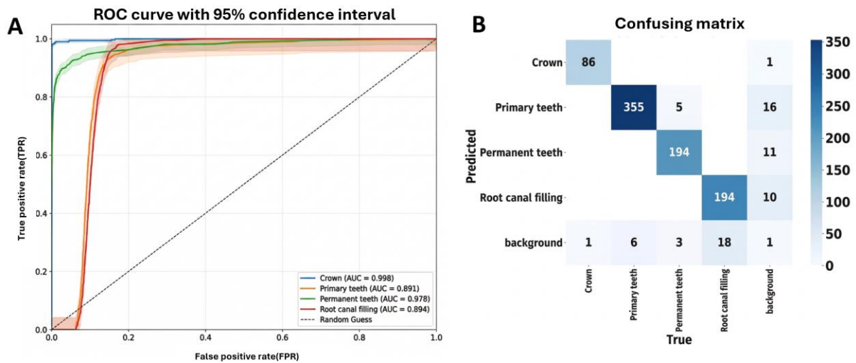
Figure 3. Comprehensive performance evaluation of the YOLO11 multitasks. (A) ROC curves and AUC values for different dental classifications. (B) Confusion matrix displaying the predicted vs. ground truth categories.
